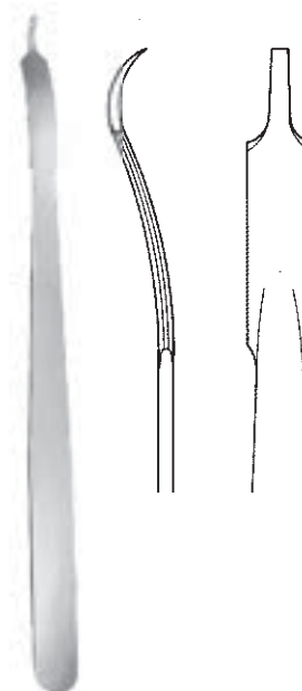
MINI-HOHMANN 4088 160mm (6.1/4") Max width: 8mm Width at tip: 2mm
